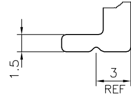
DETAIL OF "C" SCALE 3:1
