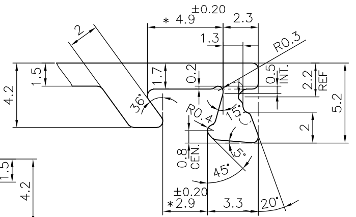
DETAIL OF "A" SCALE 4:1
