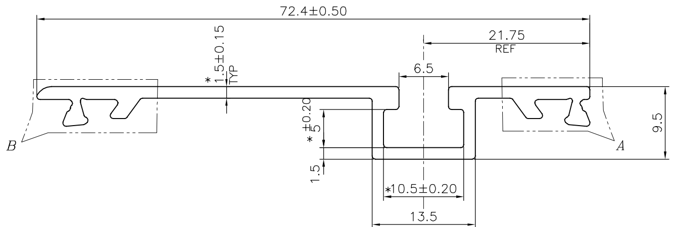
DETAIL OF "B" SCALE 4:1
