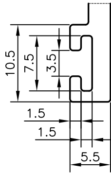
DETAIL OF "B" SCALE 2:1
