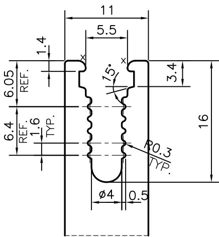
DETAIL OF "A" SCALE 2:1
