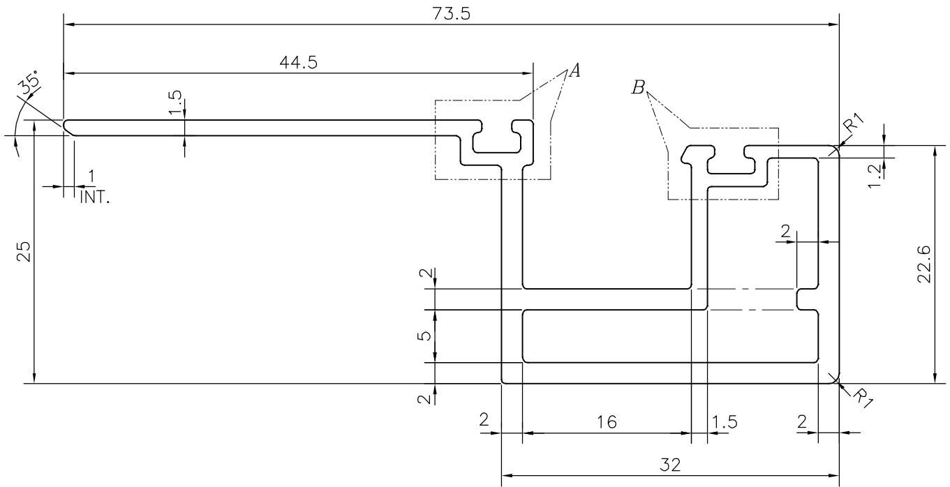
DETAIL OF "B" SCALE 3:1
