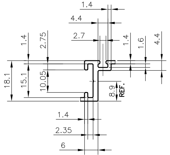
DETAIL OF "A" SCALE 1:1
