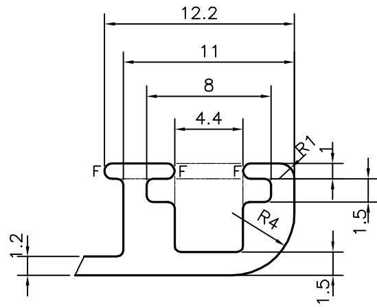
DETAIL OF "A" SCALE 3:1
