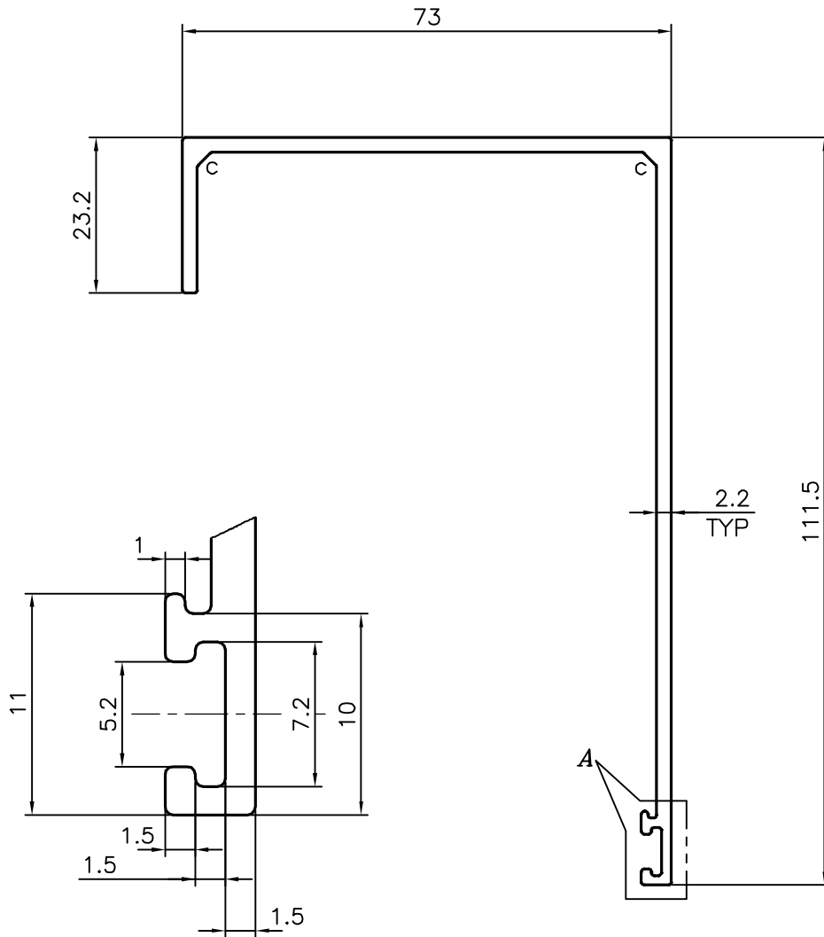
DETAIL OF "A" SCALE 3:1
