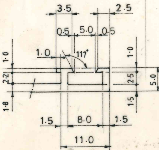
DETAIL-C
