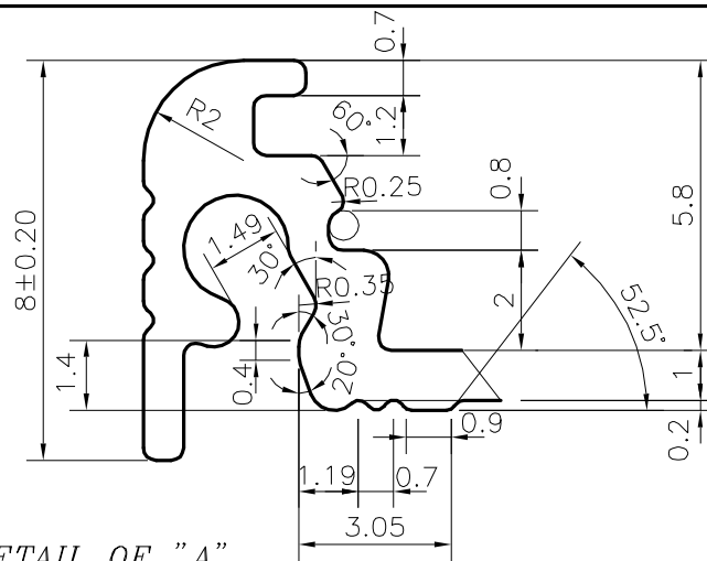
DETAIL OF "A" SCALE 6:1
