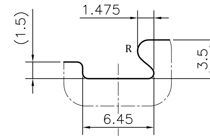
DETAIL B SCALE 3:1
