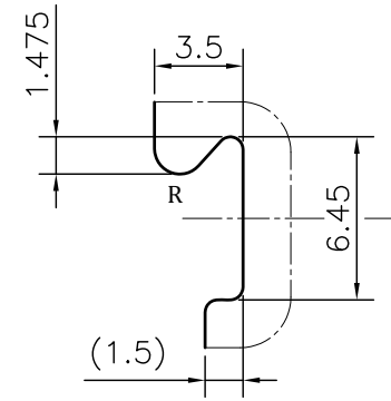
DETAIL A SCALE 3:1
