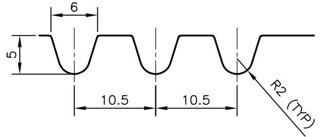
DETAIL OF "A" SCALE 2:1
