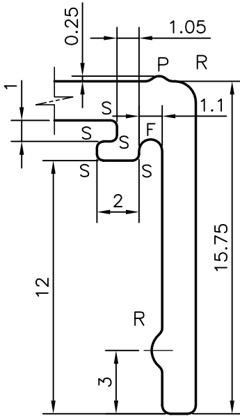
DETAIL OF "B" SCALE 4:1
