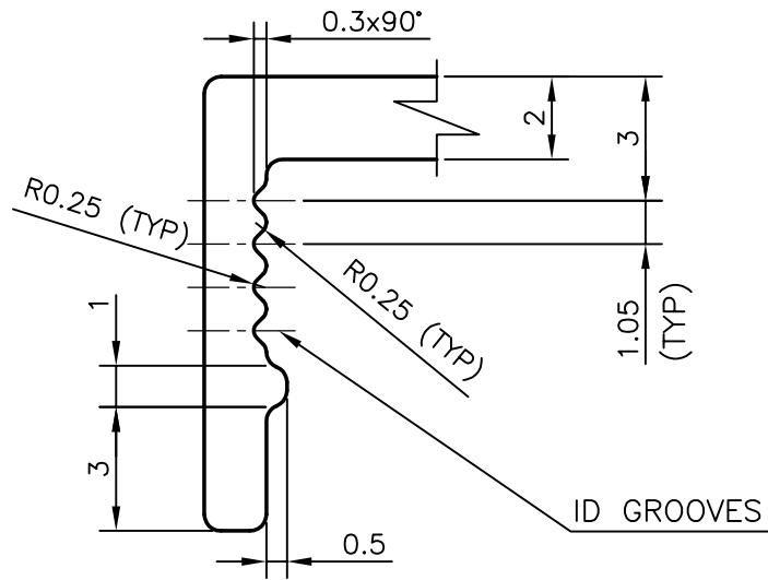
DETAIL OF "A" SCALE 5:1
