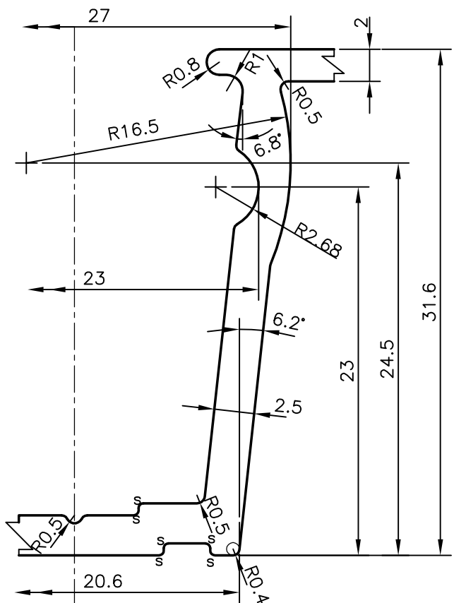
DETAIL OF "A" SCALE 3:1
