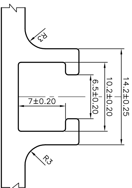
DETAIL OF "C" SCALE 5:1
