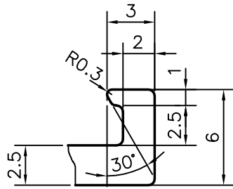
DETAIL OF "B" SCALE 3:1
