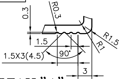
DETAIL "A" (2:1)
