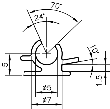
DETAIL OF "C" SCALE 2:1
