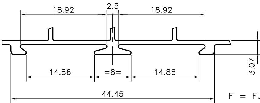
DETAIL OF "A" SCALE 2:1
