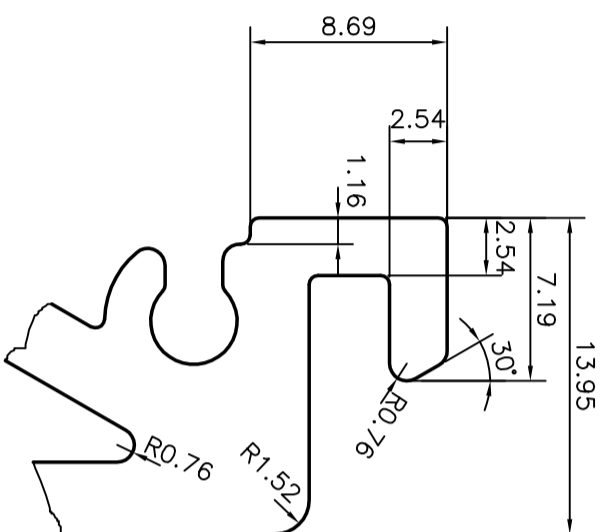
DETAIL OF "B" SCALE 3:1
