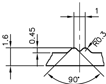
DETAIL "A" (5:1)
