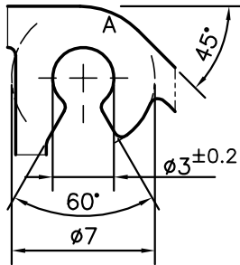
DETAIL OF "A" SCALE:- 3:1
