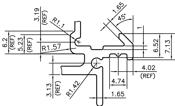
DETAILS OF "A" SCALE 2:1
