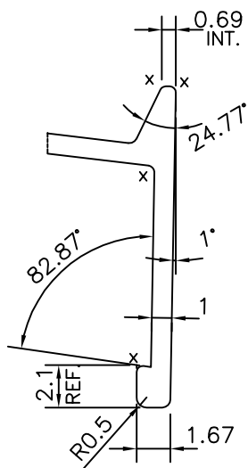
DETAIL OF "A" SCALE 3:1
