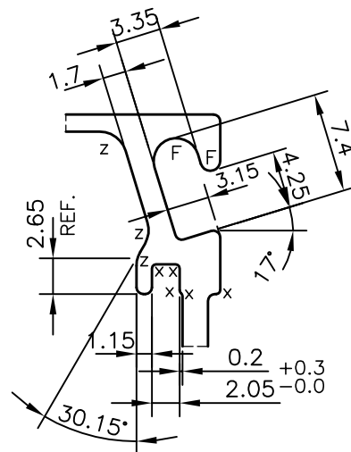
DETAIL OF "B" SCALE 2:1
