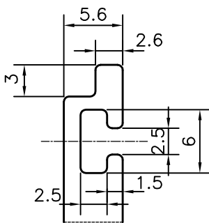
DETAIL OF "B" SCALE 2:1
