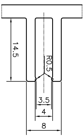
DETAIL OF "A" SCALE 2:1
