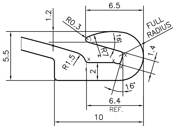
DETAIL OF "A" SCALE 4:1
