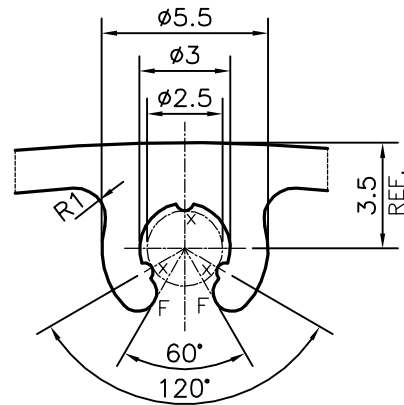
DETAIL OF "B" SCALE 4:1
