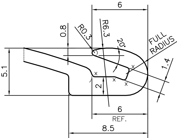
DETAIL OF "A" SCALE 4:1
