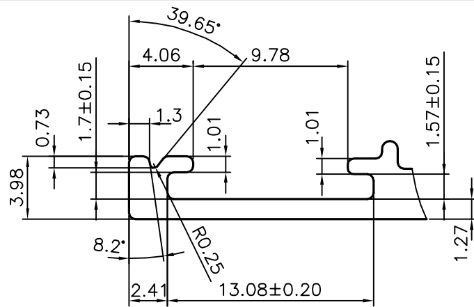
DETAIL "A" SCALE 3:1
