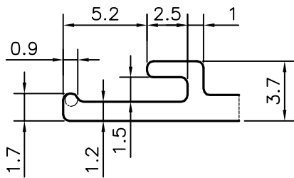
DETAIL OF "A" SCALE 3:1
