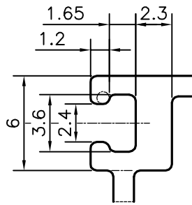
DETAIL OF "B" SCALE 3:1
