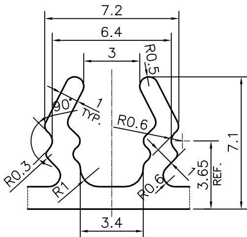
DETAIL OF "A" SCALE 5:1
