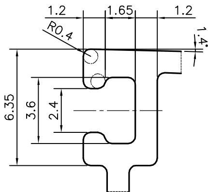
DETAIL OF "A" SCALE 5:1
