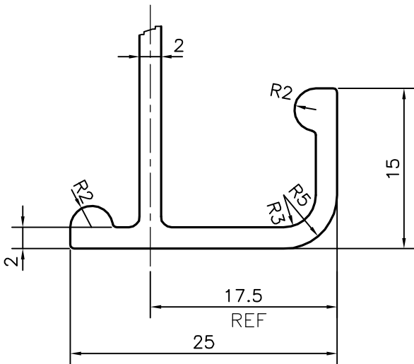
DETAIL OF "B" SCALE 2:1
