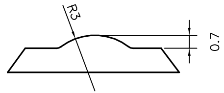
DETAIL OF "B" SCALE 5:1
