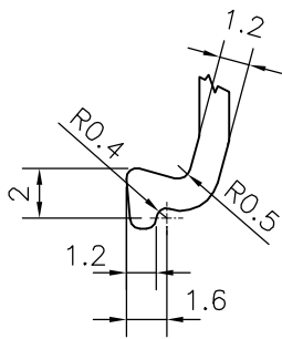
DETAIL :- A 3:1
