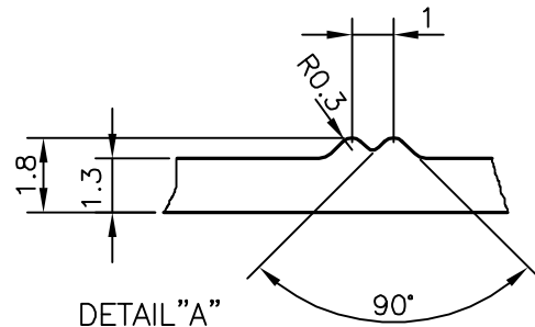
DETAIL "A" SCALE 5:1
