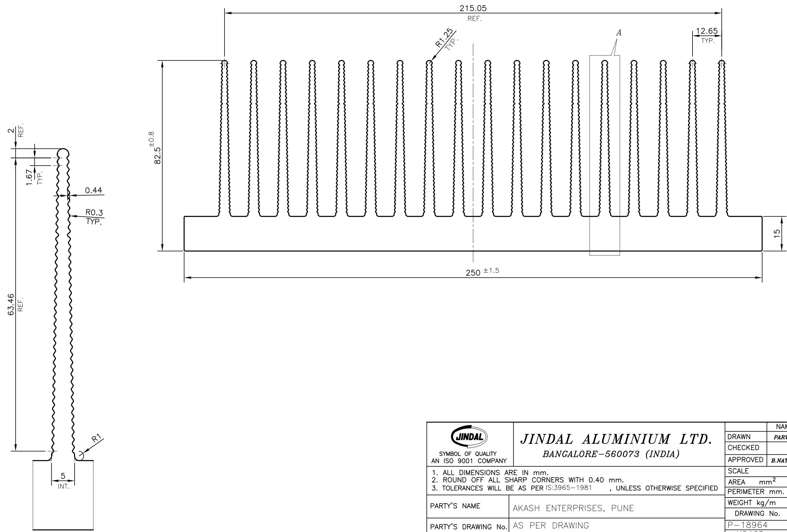
DETAIL OF "A" SCALE 2:1
