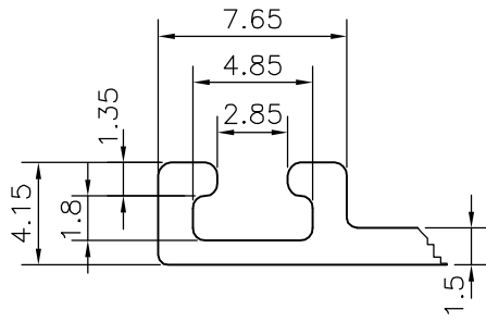
DETAIL OF "A" SCALE 3:1
