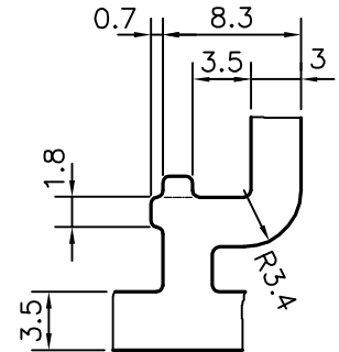
DETAIL OF "B" SCALE 2:1
