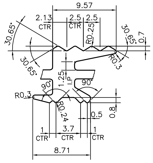
DETAIL OF "B" SCALE 3:1
