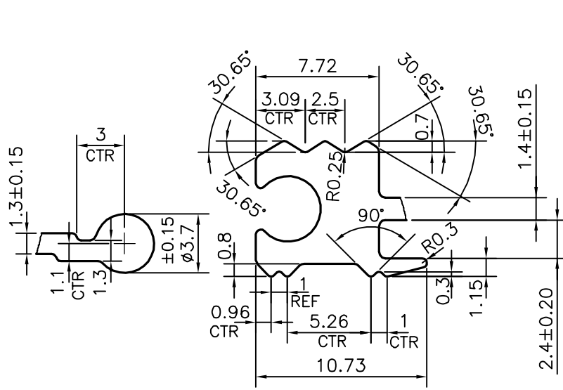
DETAIL OF "A" SCALE 3:1
