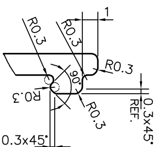
DETAIL OF "A" SCALE 4:1
