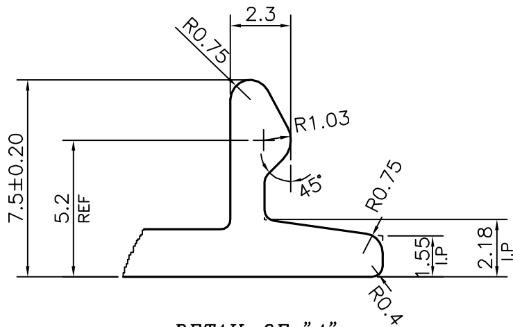
DETAIL OF "A" SCALE:- 5:1
