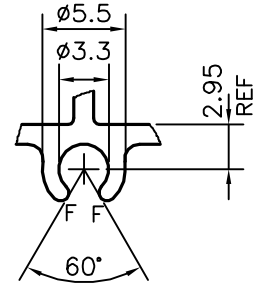
DETAIL OF "C" SCALE 2:1
