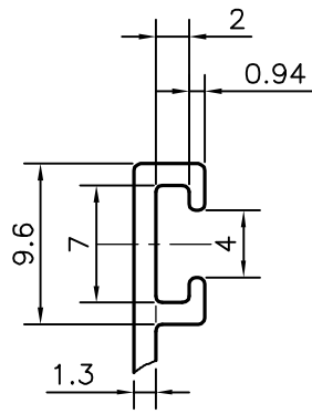
DETAIL OF "A" SCALE 2:1
