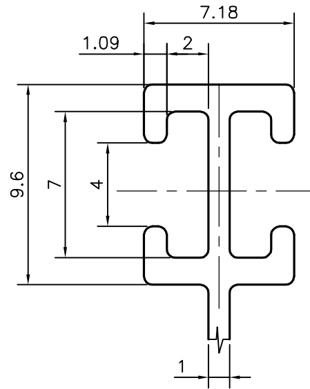
DETAILS OF "A" SCALE 4:1
