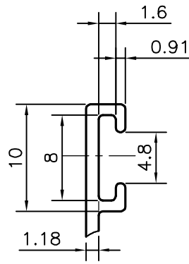
DETAIL OF "A" SCALE 2:1
