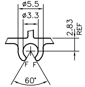
DETAIL OF "C" SCALE 2:1
