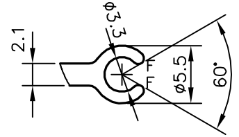
DETAIL OF "B" SCALE:- 2:1
